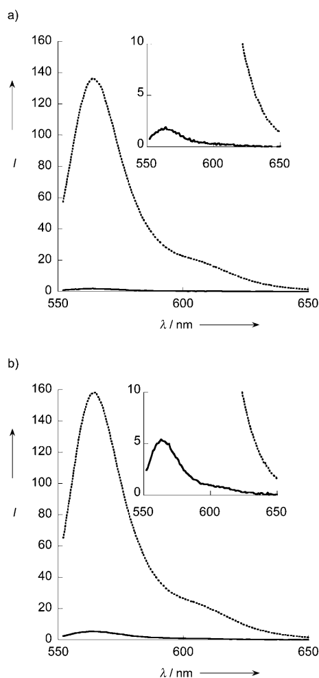
Figure 3. Fluorescence emission spectra of a) \text{MB}_{\text{MR}} and b) \text{MB}_{\text{MR}} excited at 546 nm with (·····) and without (—) the presence of Surv. Solution conditions: [\text{MB}_{\text{MR}}] = [\text{MB}_{\text{NR}}] = 0.2 \mu\text{M} , [\text{Surv}] = 0.4 \mu\text{M} , [\text{NaCl}] = 100 \text{ mM} , pH 7.0 (10 mM phosphate buffer); 20^\circ\text{C} .
