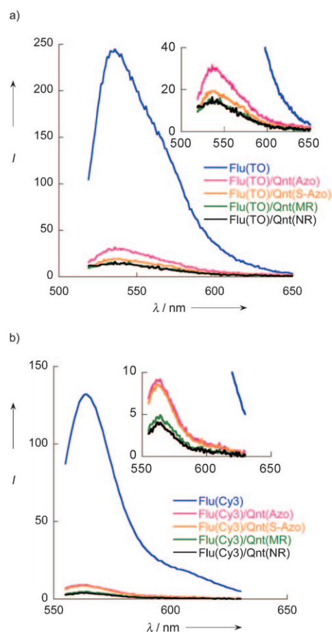
Figure 2. Fluorescence emission spectra of a) Flu(TO) excited at 516 nm and b) Flu(Cy3) excited at 546 nm, and their duplexes with Qnt(Y). Solution conditions: [Flu(X)] = 0.2 \mu M, [Qnt(Y)] = 0.4 \mu M, [NaCl] = 100 mM, pH 7.0 (10 mM phosphate buffer); 20 °C.
