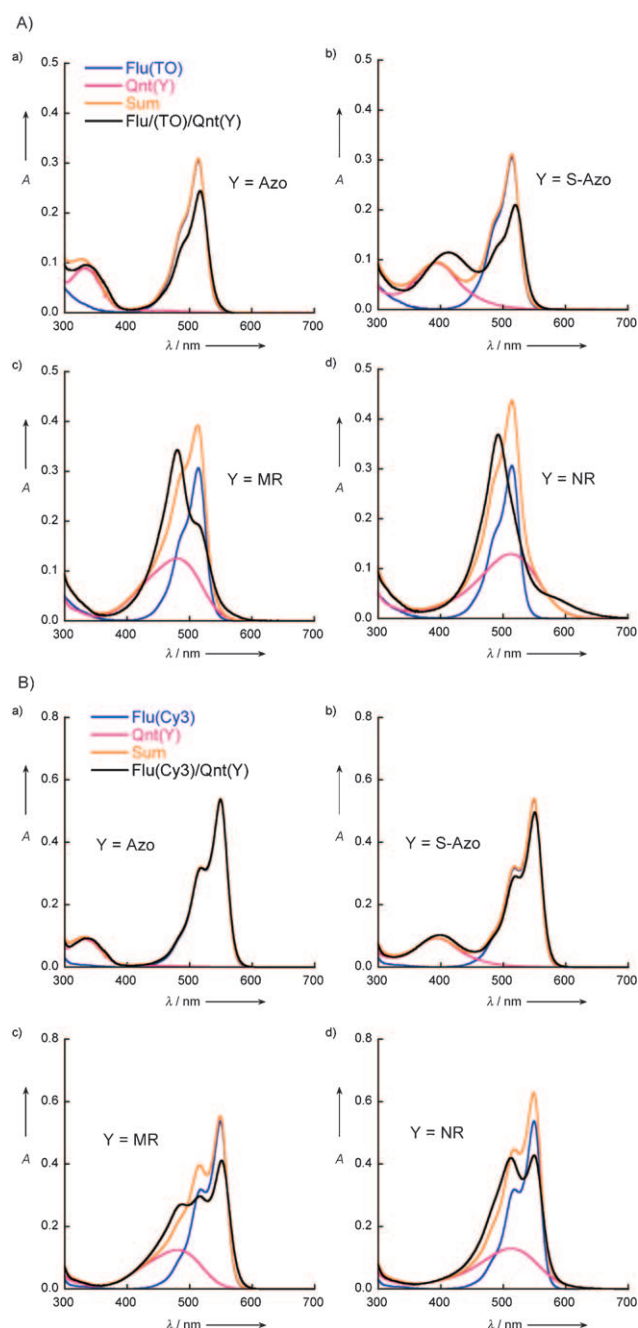
Figure 1. UV/Vis spectra of Flu(X)/Qnt(Y) with A) X = TO, B) X = Cy3. Sum: a simple sum of the spectra. Solution conditions: [Flu(X)] = 4 \mu M, [Qnt(Y)] = 4 \mu M, [NaCl] = 100 mM, pH 7.0 (10 mM phosphate buffer); 20 °C.
