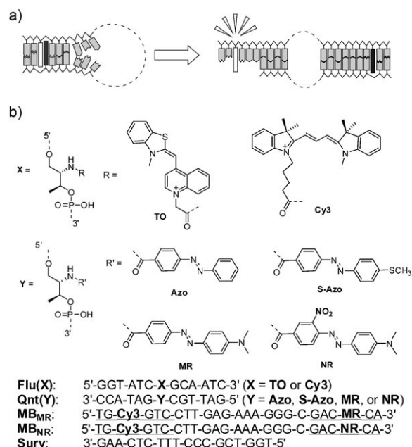
Scheme 1. a) An in-stem molecular beacon (ISMB), and b) the chemical structure of the dyes and sequences of the modified DNAs. In the MB sequences, the bases in the stem part are underlined.
