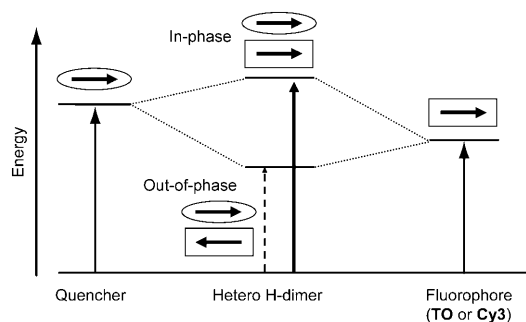
Scheme 2. Energy diagram of the heterodimer of fluorophore and quencher depicted on the basis of the exciton model. Each arrow, outlined by an ellipse or an oblong, designates the transition dipole moment.
